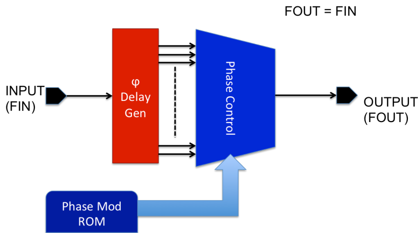
Figure 2 – SAΦIC™ Implementation of Active EMI Management
