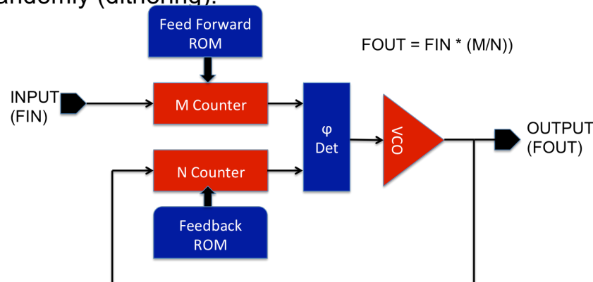
Figure 1 – PLL Based Implementation of Active EMI Management
